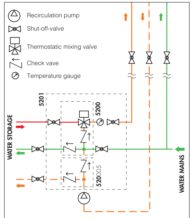
Hydraulic diagram
