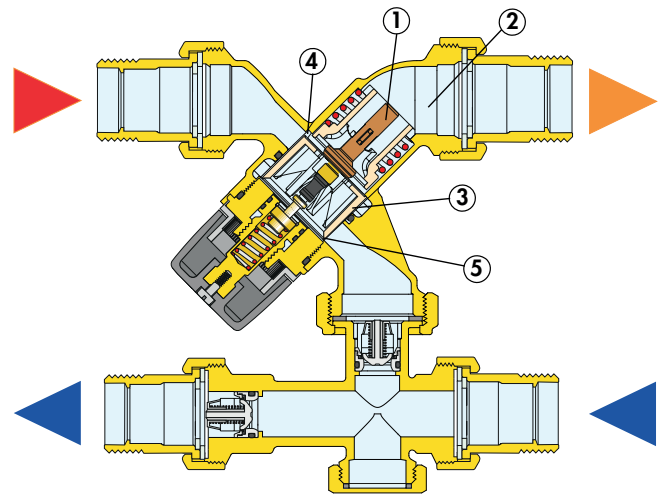
Hydraulic diagram
